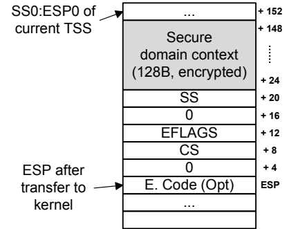
(b) Modified x86 exception frame
